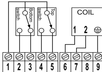
Connection (0-1 cable)
