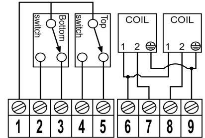
Connection (2 cable)
