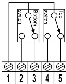
Connection (0 cable)
